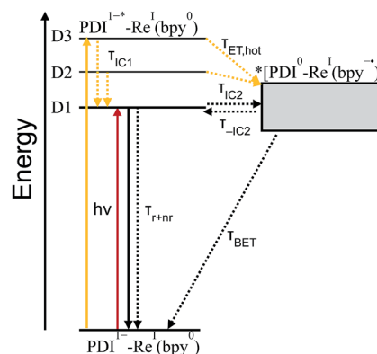
Fig. 9 Jablonski diagram showing electron transfer in PD1 1+ -Phbpy-Re-Py after excitation at 950 nm (red) or 680 nm (yellow). Energy of the charge-transfer state is shown as a range to reflect the uncertainty of the exact energy of this state.
