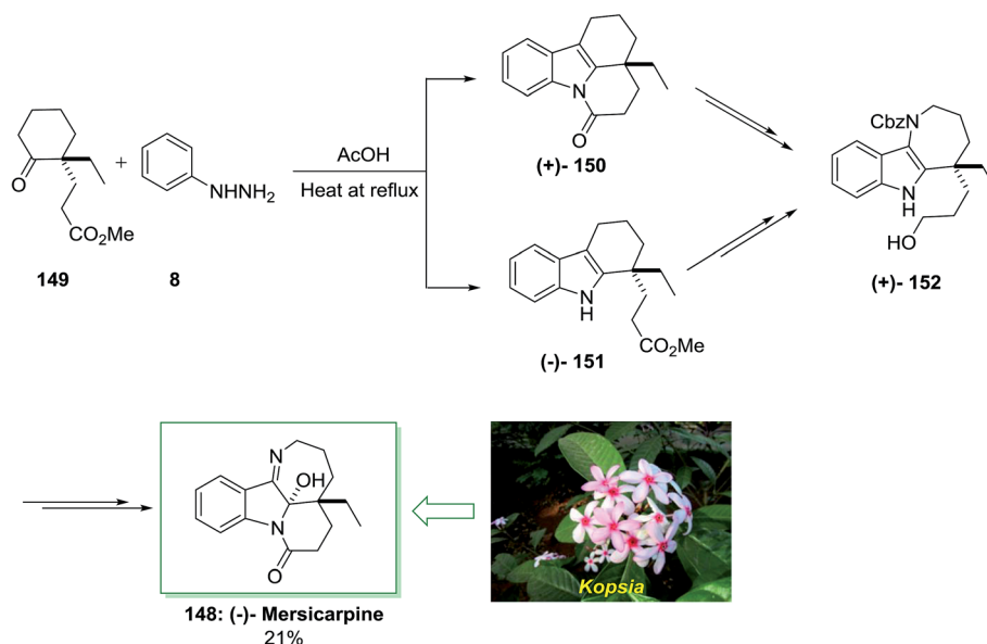
Scheme 30 Total synthesis of (–)-mescarpine 148.
