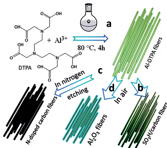
Fig. 29 Schematic illustration of the formation process of the nano-porous N-doped carbon microfibres and solid acids microfibres. [Reproduced from ref. 305 with permission from The Royal Society of Chemistry.]
