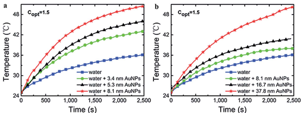
Fig. 9 The temperature changes with time for Au NPs fluids from G1 (a) and G2 (b) under 1.5 \text{ kW m}^{-2} illumination.
