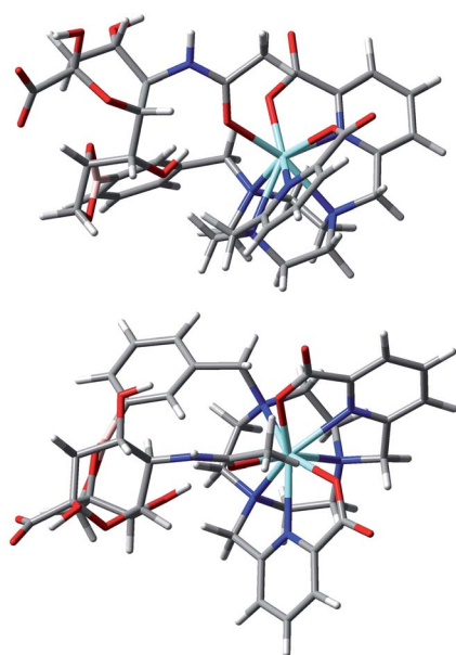
Fig. 14 Views of the hypothetical binding of the glycerol diol group to boron and cooperative ligand coordination of the amide carbonyl oxygen to the metal ion in an optimised model geometry for the complex [\text{Eu} \cdot \text{L}^3 \cdot \text{sialic acid}] . 11,12
