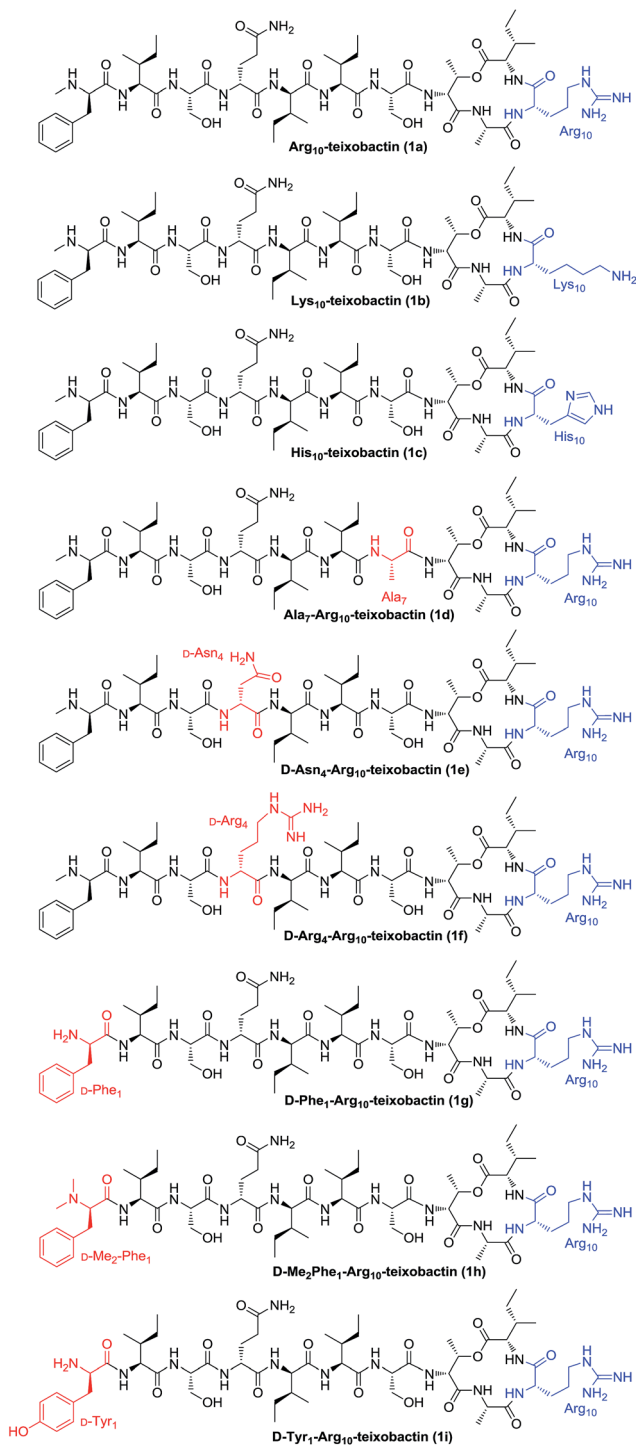
Fig. 2 Structures of teixobactin analogues 1a–1i .
