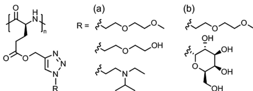
Fig. 10 Thermo-responsive poly( \alpha -glutamate)s with (a) diethylene glycol/tertiary amine side chains and (b) diethylene glycol/galactose side chains.
