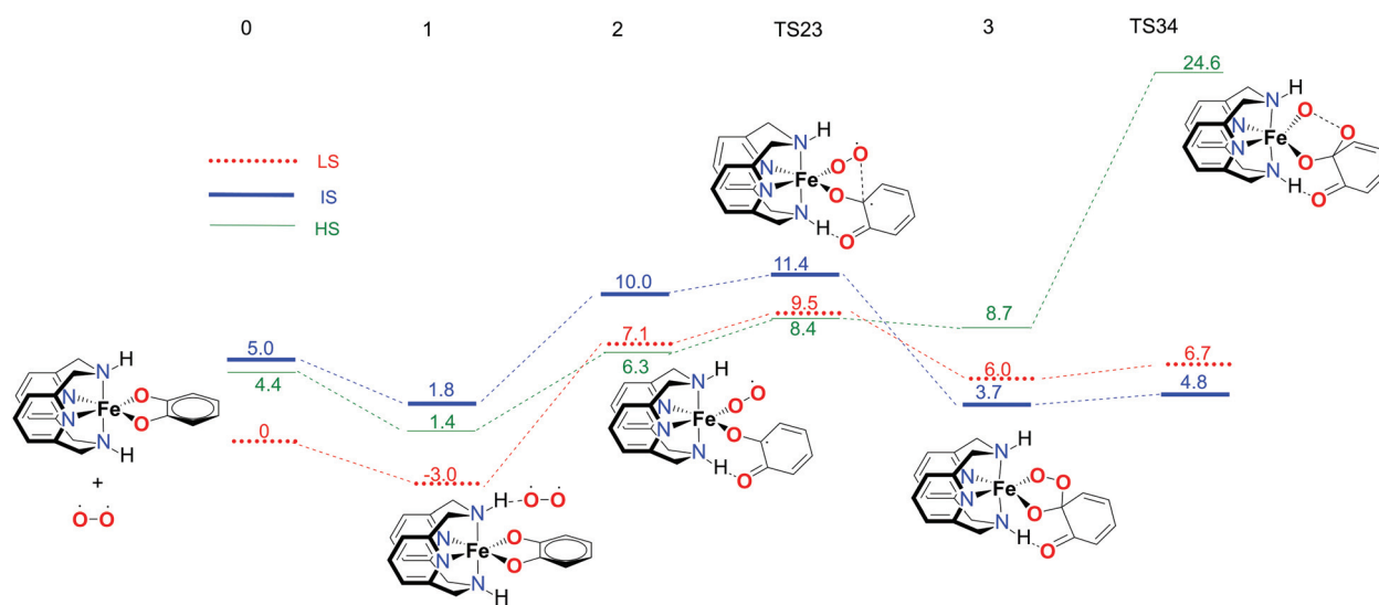
Fig. 4 Calculated reaction profile for the first part of the catechol dioxygenation mechanism, starting from the [Fe(LN 2 H 2 )(Cat)] + complex 0 . Electronic energies (kcal mol -1 ), obtained using the S12g/TZ2P level of theory, are given relative to reactants.
