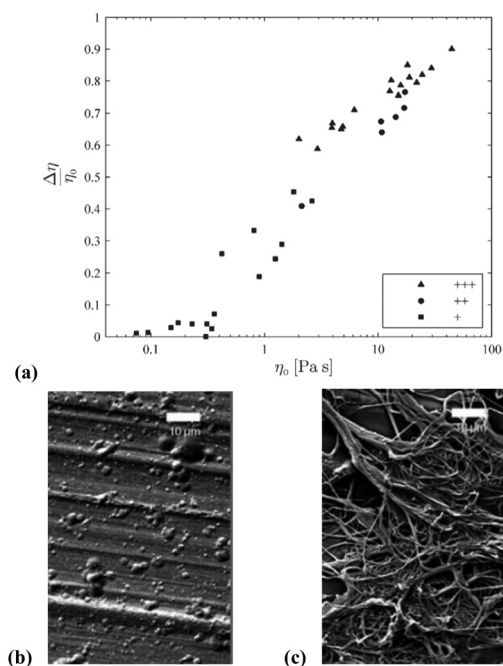
Fig. 12 (a) Relationship between shear thinning of OES–cellulose mixtures, and the propensity for fibre formation: + denotes no fibre formation; ++ denotes partial fibre formation; +++ denotes good fibre formation. Scanning Electron Microscopy (SEM) images for example '+' and '+++' cellulose electrospinning experiments are shown in (b) and (c), respectively (scale bars denote 10 µm). Reproduced and adapted with permission from J. Appl. Polym. Sci. , 2012, 125 , 1901–1909. Wiley-VCH Verlag GmbH & Co. KGaA, 2012.
