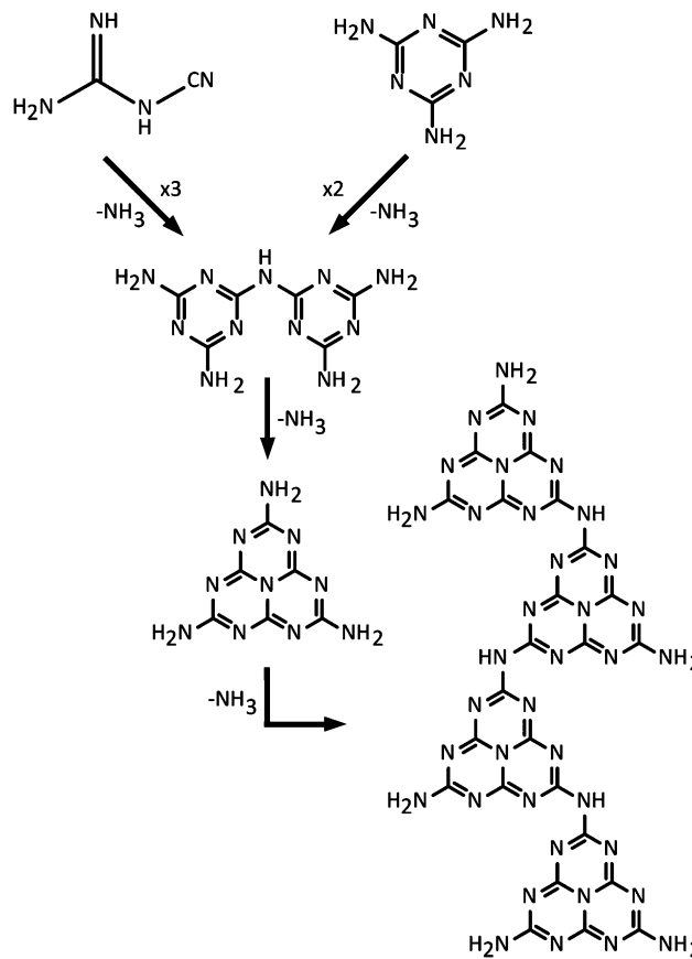
Fig. 5 Sequence of polymerization reactions proposed for dicyandiamide or melamine leading to Liebig’s melon via condensation and elimination of NH_3 components. Further condensation reactions could ultimately lead to sideways cross-linking of polyheptazine ribbons to form sheet-like structures, but no fully polyheptazine based g- C_3N_4 has been observed to date.
