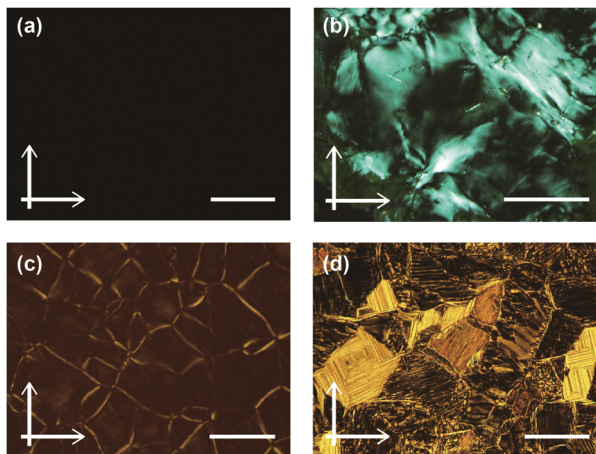
Fig. 3 Polarized optical microscopic images: (a) compound 1 in the optically isotropic LC phase (OI phase, G-form) at 25 °C; (b) compound 1 in the shear-induced mesophase (M phase, BG-form) at 25 °C; (c) compound 3 in the Col tet phase at 130 °C; and (d) compound 3 in the Col f phase at 25 °C. Scale bar: 200 μm. Arrows indicate the directions of polarizer and analyzer axes.
