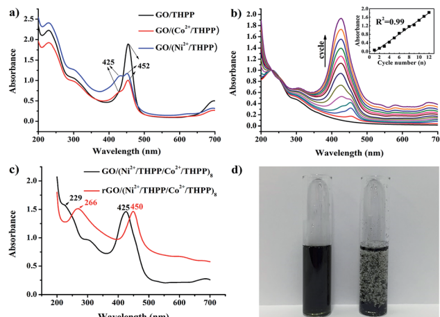
Fig. 1 (a) UV/Vis absorption spectra of \text{GO}/\text{THPP} , \text{GO}/(\text{Co}^{2+}/\text{THPP}) and \text{GO}/(\text{Ni}^{2+}/\text{THPP}) . (b) UV/Vis absorption spectra of \text{rGO}/(\text{Ni}^{2+}/\text{THPP}/\text{Co}^{2+}/\text{THPP})_n ( n = 2, 4, 6, 8, 10, 12 ). Insert: relationship of UV/Vis absorption intensity at 425 nm with increase in cycle number. (c) UV/Vis absorption spectra of \text{GO}/(\text{Ni}^{2+}/\text{THPP}/\text{Co}^{2+}/\text{THPP})_8 (before reduction) and \text{rGO}/(\text{Ni}^{2+}/\text{THPP}/\text{Co}^{2+}/\text{THPP})_8 (after reduction). (d) Solution of \text{rGO}/(\text{Ni}^{2+}/\text{THPP}/\text{Co}^{2+}/\text{THPP})_8 (left) and \text{rGO} (right) after being stored under ambient conditions for 5 months.
