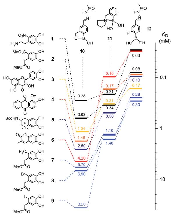
Fig. 2 Dissociation constants K_D (mM) of boronic esters obtained from catechols 1–9 and boronic acids 10–12 in MeOH/ \text{H}_2\text{O} 3 : 1 (100 mM HEPES, pH 7.8); from changes in absorption upon direct titration ( 1, 3, 4 and 6 ) or reverse titration with 4 ( 2, 5, 7–9 ).
