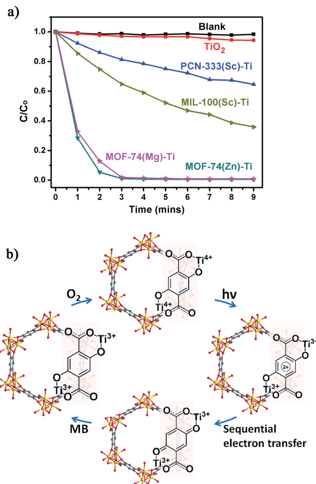
Fig. 5 (a) Photodegradation of MB using no catalyst (blank), TiO 2 , PCN-333(Sc)-Ti, MIL-100(Sc)-Ti, MOF-74(Zn)-Ti and MOF-74(Mg)-Ti with 300 W xenon light irradiation; (b) proposed mechanism of MB degradation of Ti-MOF-74 in the presence of air.
