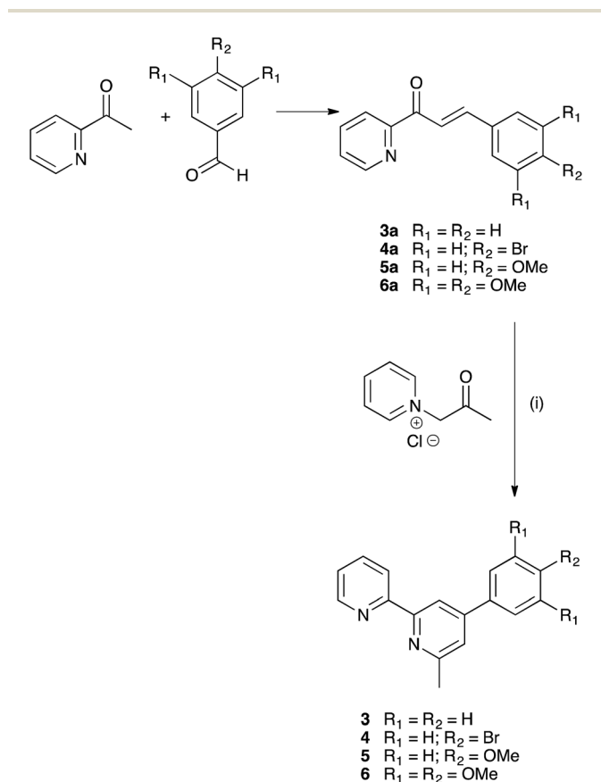
Scheme 4 Synthesis of ligands 3–6 from literature precursors 3a–6a . 16–18 Reaction conditions: (i) NH_4OAc in EtOH , reflux.
