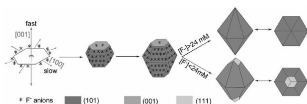
Scheme 2 Sketch of the growth mechanism of dodecahedral and octodecahedral α-Fe 2 O 3 particles (modified with permission from ref. 51, copyright 2010 Wiley-VCH).
