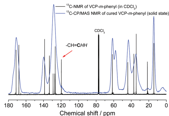
Fig. 5 13 C-NMR comparison: 13 C NMR ( \text{CDCl}_3 , 75 MHz) of un-cured VCP- m -phenyl and 13 C-CP/MAS NMR (100 MHz) of cured VCP- m -phenyl. The signal at 119.7 ppm defines the carbon atom of the terminal vinyl bond. After curing within the 13 C-CP/MAS NMR spectra only a shoulder, hardly perceived at 119.7 ppm, is observed, which indicates a high cross-linking density of the cured VCP- m -phenyl.
