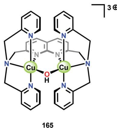
Fig. 55 Structure of the dinuclear Cu II,II complex [Cu 2 II,II (bpman)(μ-OH)] 3+ ( 165 ). bpman = 2,7-[bis(2-pyridylmethyl)aminomethyl]-1,8-naphthyridine.
