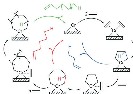
Scheme 1 Metallacyclic mechanism for selective ethylene oligomerisation.
