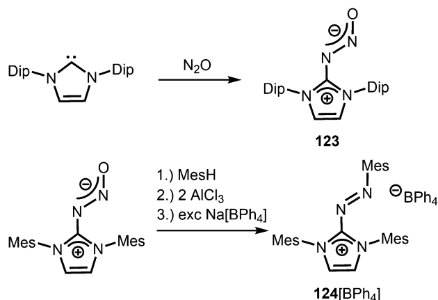
Scheme 28 Synthesis of representative examples for the compound classes: diazotates ( 123 ) and azoimidazolium salts ( 124 [\text{BPh}_4] ).
