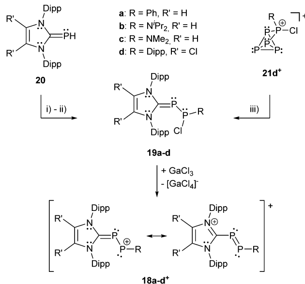
Scheme 7 Two different approaches for the synthesis of NHC stabilized chlorodiphosphanes 19a–d comprising bonding motif B. For 19a,b : (i) + \text{R}(\text{P})\text{Cl}_2 , +DABCO, −DABCO*HCl; for 19c : (ii) +2 \text{PCl}(\text{NMe}_2)_2 , +DABCO, −DABCO*HCl, − \text{P}(\text{NMe}_2)_3 ; for 19d : (iii) +3 1,3-bis(2,6-diisopropylphenyl)-4,5-dichloro-imidazole-2-ylidene, −5 + . Subsequent chloride abstraction yields polarized cationic diphosphenes 18a–d + . Only two resonance structures that indicate the polarization of 18a–d + are shown.
