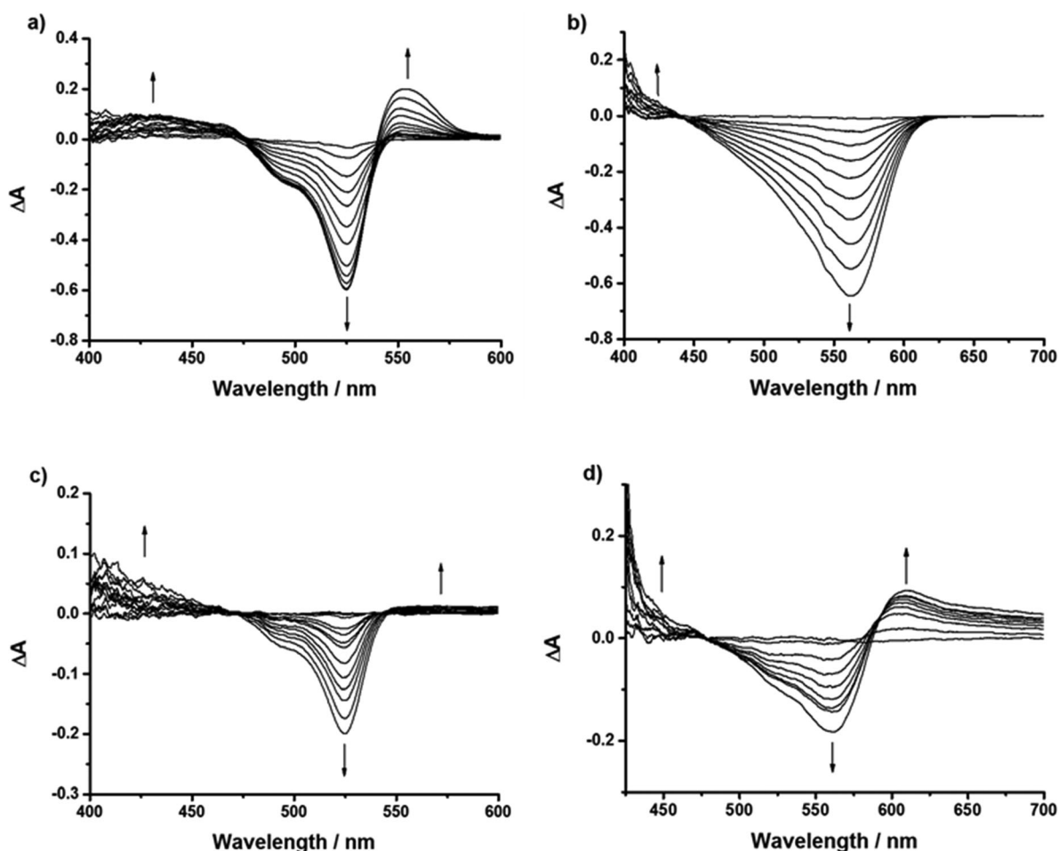
Fig. 9 UV-visible difference spectra recorded in CH 2 Cl 2 containing [Bu 4 N][ClO 4 ] (0.5 M) using spectroelectrochemical methods showing the inter-conversion of (a) 4 to 4 •+ , (b) 5 to 5 •+ , (c) 4 to 4 1+ and (d) 5 to 5 1+ at 248 K. Arrows indicate the progress of the oxidation or reduction.
