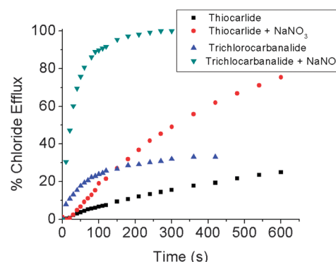
Fig. 1 Chloride efflux caused by the addition of the antibiotics thiocarlidide or trichlorocarbanalidide (0.675 mol%), with and without NaNO 3 added to the exterior of POPC vesicles loaded with 0.5 M NaCl, 0.1 M Na 2 SO 4 , and 20 mM phosphate buffer, pH = 7.2. 100% chloride efflux was determined by lysing the liposomes with Triton X.
