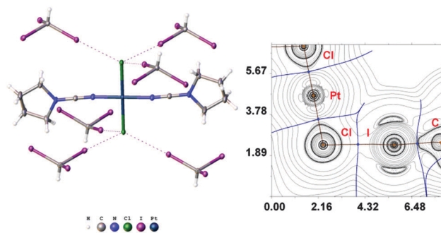
Fig. 5 Left: View of fragment 3 ·( \text{CHI}_3 ) 6 from 3 ·2 \text{CHI}_3 . Thermal ellipsoids are shown with 50% probability and short contacts are indicated by dotted lines. Coordinates of this fragment were applied in further DFT calculations. Right: Contour line diagram of the Laplacian distribution \nabla^2\rho(r) (cross-section along the plane Pt–Cl–I) was received as a result of the topological analysis of the electron density distribution in the model structure. Bond paths are shown as brown lines, selected zero-flux surfaces – as blue lines, bond critical points (3, –1) are shown in blue, nuclear critical points (3, –3) – in pale brown, length unit – Å.
