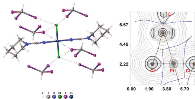
Fig. 3 Left: View of fragment 4 ·( \text{CHI}_3 ) 6 from 4 ·2 \text{CHI}_3 . Thermal ellipsoids are shown with 50% probability and short contacts are indicated by dotted lines. Coordinates of this fragment were applied in further DFT calculations. Right: Contour line diagram of the Laplacian distribution \nabla^2\rho(r) (cross-section along the plane Pt–Cl–I) was received as a result of the topological analysis of the electron density distribution in the model structure. Bond paths are shown as brown lines, selected zero-flux surfaces – as blue lines, bond critical points (3, –1) are shown in blue, ring critical points (3, +1) – in orange, nuclear critical points (3, –3) – in pale brown, length unit – Å.
