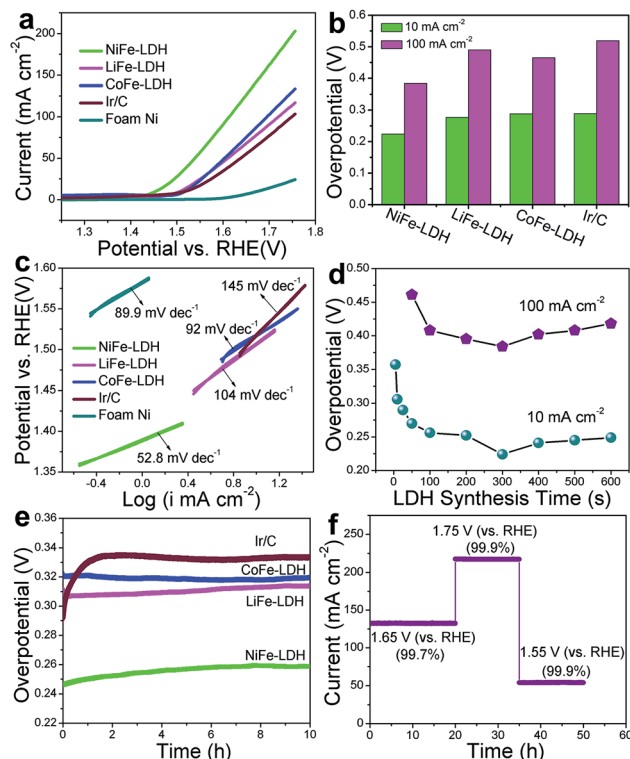
Fig. 3 (a) Linear sweep voltammetric (LSV) curves, (b) overpotential (at 10 and 100 mA cm -2 ) and (c) Tafel plots of the MFe-LDH (M = Ni, Co and Li) nanoplaleet arrays and the commercial electrocatalyst Ir/C; (d) overpotentials (at 10 and 100 mA cm -2 ) of NiFe-LDH nanoplaleet arrays synthesized for various durations from 0 s to 600 s; (e) chronopotentiometric measurements at 10 mA cm -2 for the MFe-LDH (M = Ni, Co and Li) nanoplaleet arrays and commercial Ir/C for 10 h; (f) chronoamperometric curve at varied overpotentials for the NiFe-LDH nanoplaleet array.
