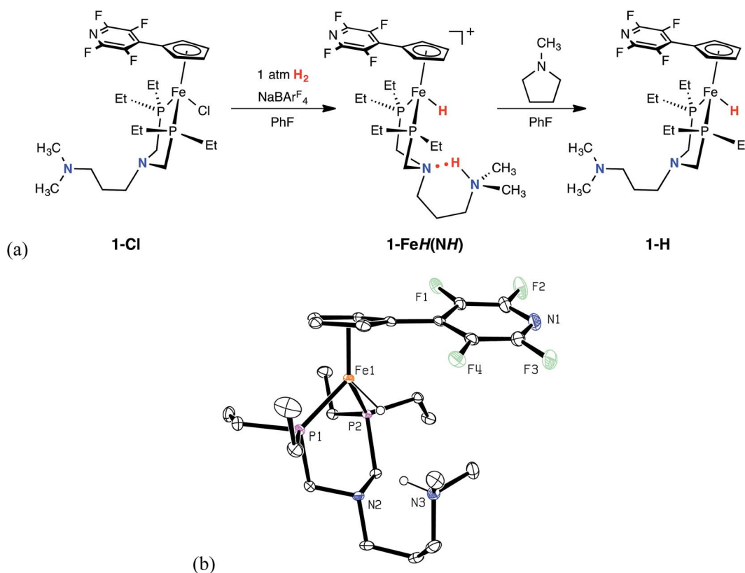
Fig. 1 (a) Observable catalytic intermediates from the reaction of 1-Cl with NaBAR 4 F under 1 atm H 2 . (b) Representation of the solid-state structure of 1-FeH(NH) with 30% probability ellipsoids. The BAR 4 F anion and all hydrogen atoms with the exception of the proton and the hydride are omitted for clarity.
