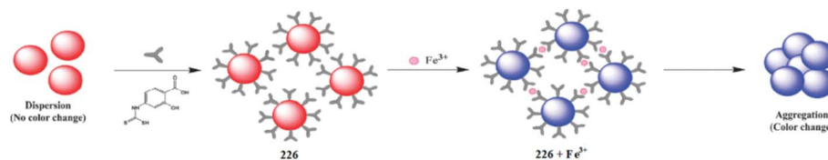
Fig. 190 Schematic for the colorimetric sensing of Fe 3+ using DTC-PAS-Au NPs 226 as colorimetric probes.
