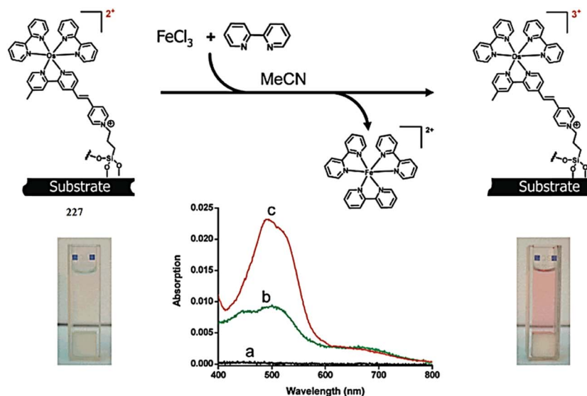
Fig. 191 In situ absorption spectral change after treating the 227-based monolayer on glass with 5 ppm of FeCl 3 in dry CH 3 CN and subsequently trapping the formed Fe 2+ with excess bipy to afford [Fe(bipy) 3 ] 2+ : (a) baseline (black), (b) 227-based monolayer in dry CH 3 CN with bipy (green), (c) in situ generation of [Fe(bipy) 3 ] 2+ (red) (a–c in figure); the images of the vials indicate the colorimetric change in the reaction solution before and after treatment with ferric ions.
