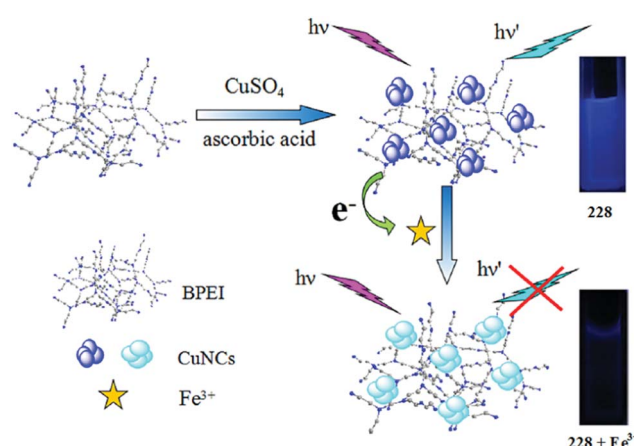
Fig. 192 Synthetic strategy of the BPEI–CuNCs and the mechanism of the BPEI–CuNCs probe for Fe 3+ sensing.
