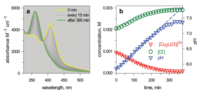
Fig. 15 (a) Spectra taken on a 1 mm quartz cuvette containing 1.1.1-cryptand ( 14 , ca. 0.1 M), [\text{Cu}_2(\text{L})]^{4+} ( \text{L} = \text{10} , 3 \times 10^{-3} M), KCl ( 3 \times 10^{-3} M) and triflic acid to adjust the \text{pH}_{\text{init}} to 6; (b) symbols: values of [\text{Cu}_2\text{L}(\text{Cl})]^{3+} and [\text{Cl}^-] obtained from the spectrophotometric titration through appropriate algorithms; lines: calculated concentration profiles when the pH increases at a rate of 1.0 \times 10^{-4} unit \text{s}^{-1} . 25
