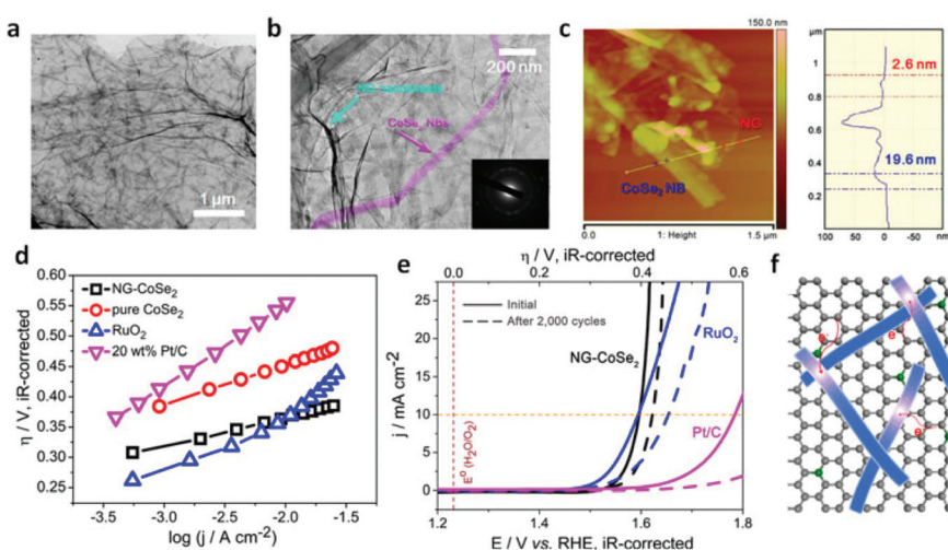
Fig. 14 (a–b) TEM images with different magnifications of NG– \text{CoSe}_2 composite. The inset in (b) shows the corresponding SAED pattern. (c) AFM image and corresponding height profile of NG– \text{CoSe}_2 composite. (d–e) Tafel plot and polarization curves for OER on bare GC electrode and modified GC electrodes comprising the NG sheets, commercial 20 wt% Pt/C and \text{RuO}_2 catalysts, pure \text{CoSe}_2 nanobelts, and NG– \text{CoSe}_2 composite. (f) Schematic image demonstrates the electron donation from the NG to \text{CoSe}_2 . Gray, green balls and blue belts correspond to C, N atoms and \text{CoSe}_2 nanobelts, respectively (reproduced with permission from ref. 44. Copyright 2014 American Chemical Society).
