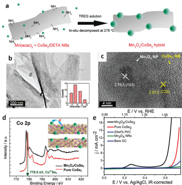
Fig. 13 (a) Polyol synthesis with \text{CoSe}_2/\text{DETA} NBs to generate \text{Mn}_3\text{O}_4/\text{CoSe}_2 hybrid. (b) TEM images of \text{Mn}_3\text{O}_4/\text{CoSe}_2 hybrid prepared at 278 °C for 1 h. The inset in (b) shows the corresponding particle-size histogram. (c) HRTEM image of an attached nanoparticle and its neighboring \text{CoSe}_2 support. (d) Co 2p XPS spectra for pure \text{CoSe}_2/\text{DETA} NBs and as constructed \text{Mn}_3\text{O}_4/\text{CoSe}_2 hybrid. Inset demonstrates the electron donation from the \text{Mn}_3\text{O}_4 to \text{CoSe}_2 . Pink and yellow balls correspond to Co and Se atoms, respectively. (e) Polarization curves for OER on bare GC electrode and modified GC electrodes comprising the \text{Mn}_3\text{O}_4 NRs, 20 wt% Pt/C, pure \text{CoSe}_2/\text{DETA} NBs and \text{Mn}_3\text{O}_4/\text{CoSe}_2 hybrid, respectively (reproduced with permission from ref. 42. Copyright 2012 American Chemical Society).
