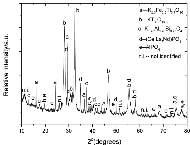
Fig. 14 X-ray powder diffraction pattern of the reaction product formed as a result of chemical reaction between K_2CO_3 and FeTiO_3 at 825^\circ C for 4 hours in air. The main phases compare well with the ICDD references: 00-041-1100 K_2O \cdot 8TiO_2 , 00-040-0960 K_{2.3}Fe_{2.3}Ti_{5.7}O_{16} , 00-032-0731 K_{1.25}Al_{1.25}Si_{0.75}O_4 , 00-046-1295 (Ce, La, Nd)PO_4 and 04-009-5769 Al(PO_4) .
