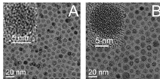
Fig. 22 TEM images of (A) core-only \text{NaYF}_4:\text{Yb,Er} UCNP s and (B) core-shell UCNP s \text{NaYF}_4:\text{Yb,Er}@\text{NaYF}_4 . The increase in diameter is attributed to the growth of an undoped host material shell on the surface of the core-only UCNP s. Reprinted with permission from ref. 70. Copyright © 2007, American Chemical Society.
