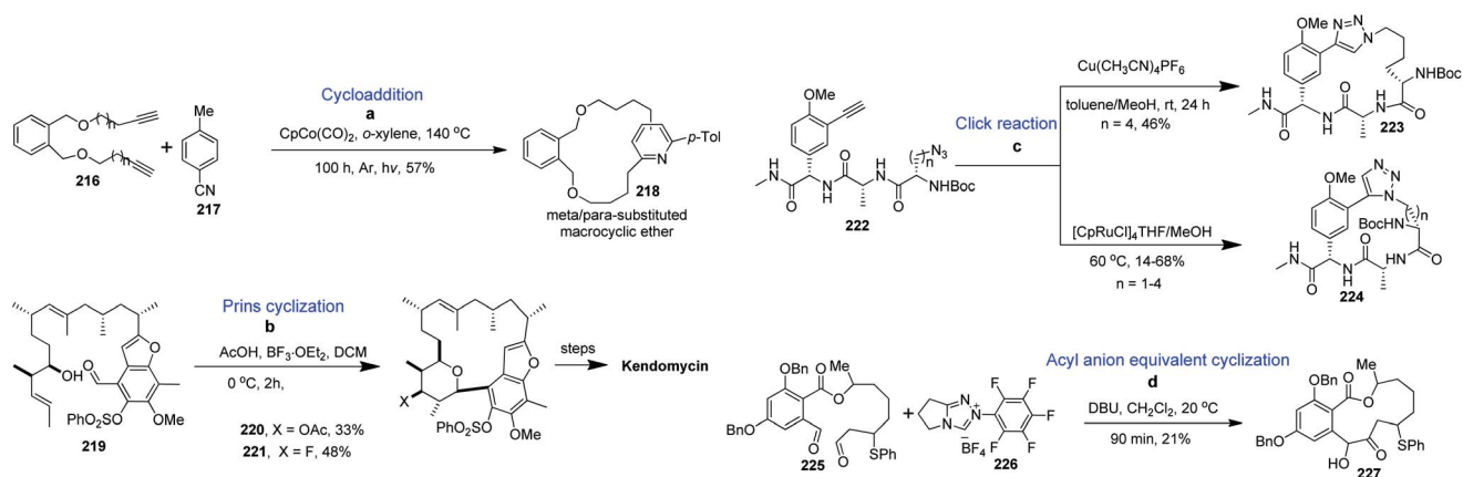
Scheme 8 Synthesis of benzannulated cyclic compounds via cycloaddition, Prins cyclization, click chemistry and acyl anion equivalent macrocyclization strategies.
