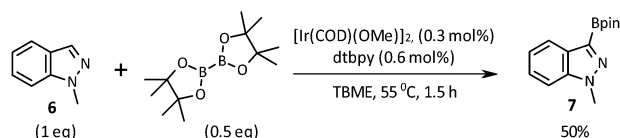
Scheme 2 Borylation of 1-Me-1H-indazole with B 2 Pin 2 .
