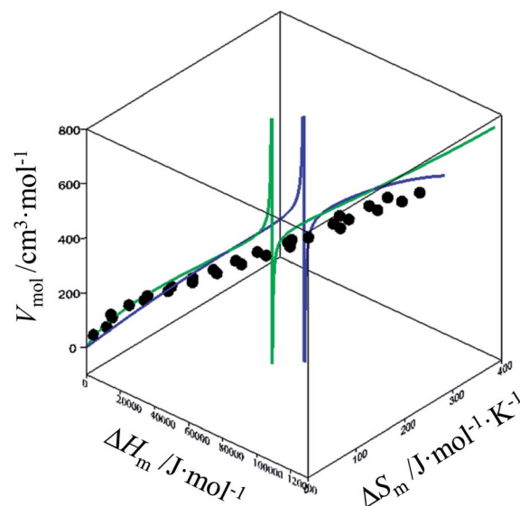
Fig. 7 Three-dimensional V_{\text{mol}} , \Delta H_m , \Delta S_m plot for linear alkanes fitted with a parabolic H/S function (blue trace) or a reciprocal Hill plots (green trace). An asymptotic behaviour is expected to occur when the melting temperature approaches the selected reference temperature T^0 = 298.15 \text{ K} .
