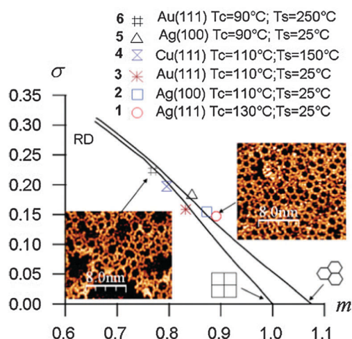
Fig. 7 (m, \sigma) Diagram of the minimal spanning tree (MST) statistical analyses for different BDBA polymer networks. T_c refers to the deposition flux ( 90^\circ\text{C} = low flux, 110^\circ\text{C} = high flux) and T_s refers to the substrate temperature during deposition. Adapted from ref. 15, copyright (2011) American Physical Society.
