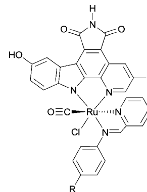
16a R = H ( \Delta -FL172) \text{IC}_{50} = 130 nM 16b R = CH 3 ( rac -FL224) 4% inhibition at 100 nM 16c R = F ( rac -FL252) no inhibition at 100 nM
