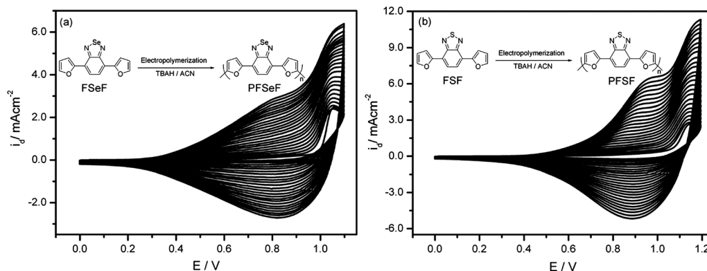
Fig. 4 Electropolymerization of (a) 2.3 \times 10^{-3} M of FSeF and (b) 3.1 \times 10^{-3} M of FSF in 0.1 M TBAH/ACN at a scan rate of 100 mV s -1 by potential scanning to give PFSeF and PFSF , respectively.
