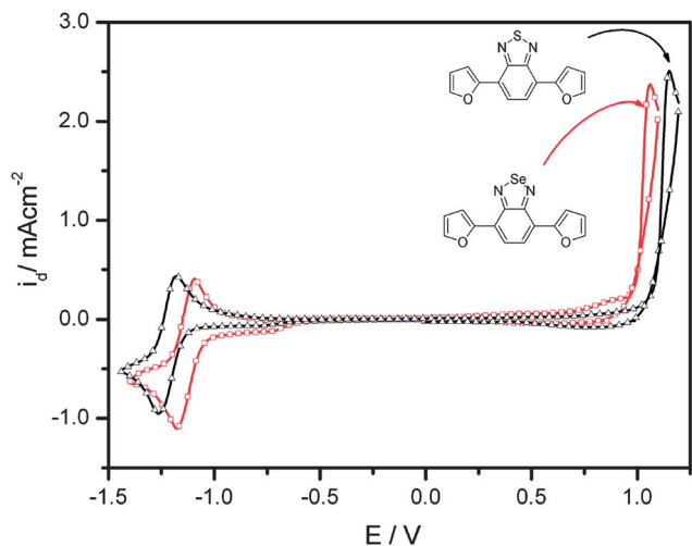
Fig. 3 Cyclic voltammograms of 3.3 \times 10^{-3} M of FSeF and 4.1 \times 10^{-3} M of FSF in 0.1 M TBAH/ACN electrolyte solution at a scan rate of 100 mV s -1 vs. Ag/AgCl.
