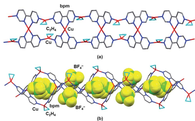
Fig. 3 X-Ray crystal structure of complex 3 encapsulating BF 4 − anions.
