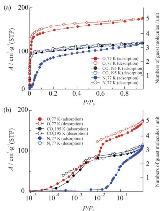
Fig. 4 (a) Adsorption (filled circles) and desorption (open circles) isotherms of 2 for O 2 (red) at 77 K, CO 2 (black) at 195 K and N 2 (blue) at 77 K. (b) Adsorption and desorption isotherms plotted against the logarithmic relative pressure.
