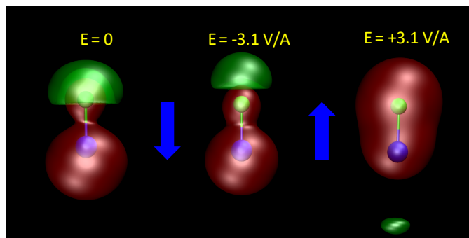
Figure 9: The QM response of a NaCl molecule in an applied electric field E = \pm 3.1 \text{ V/\AA} (field direction indicated by blue arrows). The resulting potential isosurfaces (red = positive, green = negative) and total dipole moments are: V = \pm 2 \text{ V} and \mu = 9 \text{ D} (left), V = \pm 3.5 \text{ V} and \mu = 14.3 \text{ D} (middle), V = \pm 3.5 \text{ V} and \mu = -24.7 \text{ D} (right). QM level: B3LYP/aug-cc-pvdz.
