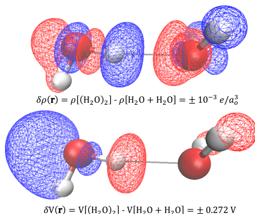
Figure 11: Deformation densities \delta\rho(\mathbf{r}) (top) and electric potentials \delta V(\mathbf{r}) (bottom) when two water molecules are brought together: \text{H}_2\text{O} + \text{H}_2\text{O} \rightarrow (\text{H}_2\text{O})_2 . The blue and red isosurfaces denote increases (+) and decreases (-), respectively. Small changes in electron density yield large changes in electric potentials. QM level: B3LYP/6-31+G*.
