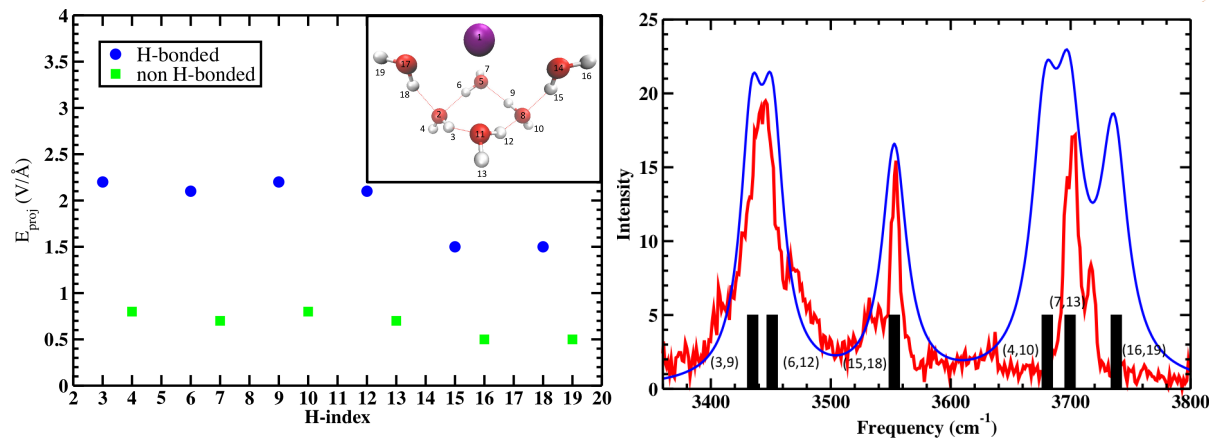
Figure 4: (Left) Projected QM E fields (left) on the H atoms in \text{Cs}^+(\text{H}_2\text{O})_6 where the blue and green symbols denote those OH groups that are H-bonded and free, respectively (the H-indices correspond to those in the inset). (Right) Comparison of the measured vibrational spectra (red) and that from the projected QM fields (black bars) and Lorentzian fits to QM fields (blue). See Wolke et al. 56 for more details. QM level: MP2/aug-cc-pVDZ.
