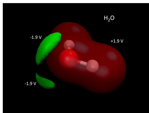
Figure 5: QM electric potentials of \text{H}_2\text{O} . Electric potential isosurfaces are: +1.9\text{ V} (red) wrapping around the entire molecule, and -1.9\text{ V} (green) corresponding to the lone pairs of electrons. QM level: MP2/aug-cc-pVDZ
