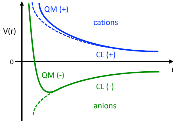
Figure 2: Illustration of the differences between the of electric potentials of an atomic QM cation (blue) and anion (green) vs. CL \pm unit point charges.
