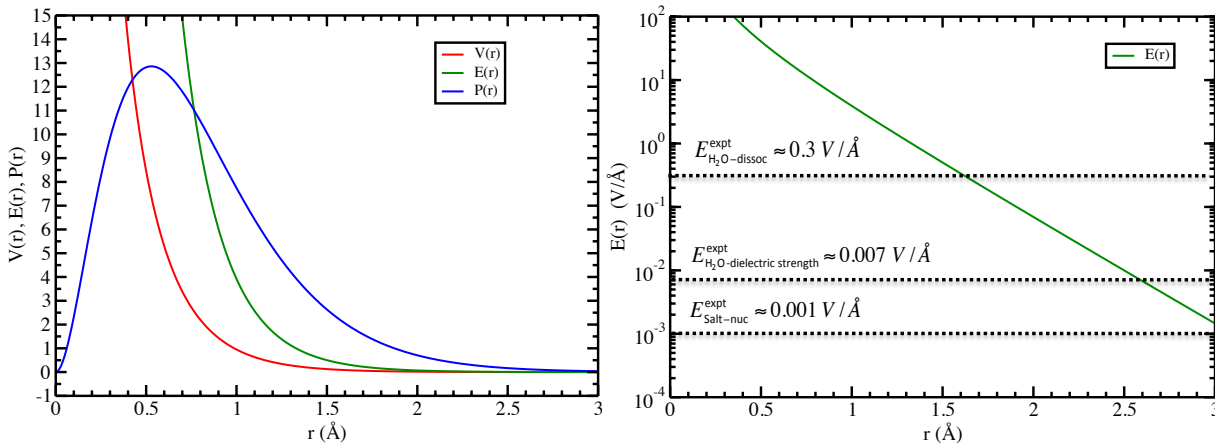
Figure 1: Quantum electric potential V(r) , field E(r) , and scaled radial probability 4\pi P(r) for the “neutral” hydrogen atom (left), and (right) a few reference field strengths compared to that from hydrogen (note vertical log-scale): for \text{H}_2\text{O} dissociation, \text{H}_2\text{O} dielectric strength, and that required to induce KCl salt nucleation.
