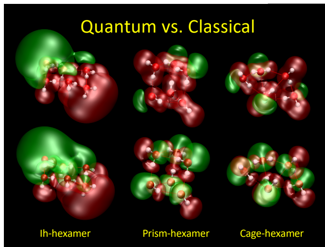
Figure 7: Comparison of electric potentials of quantum mechanical (top) vs. classical SPC/E point charge (bottom) description of three energetic minima for (\text{H}_2\text{O})_6 . O and H atoms are red and white, respectively. Electric potential isocontours are: +1.4 V (red), -1.4 V (green). QM level: HF/6-31++G**
