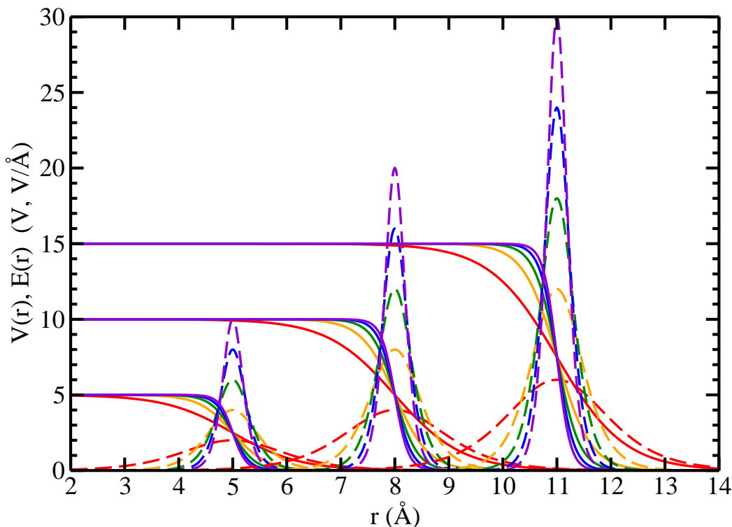
Figure 13: Comparison of interfacial electric potentials (solid) and corresponding fields (dashed) for different MIPs ( V_o = 5, 10, 15 V), interface locations ( R = 5, 8, 11 \text{ \AA} ), and width parameters ( k = 0.8 (red), 1.6 (orange), 2.4 (green), 3.2 (blue), 4.0 (purple) \text{\AA}^{-1} ).
