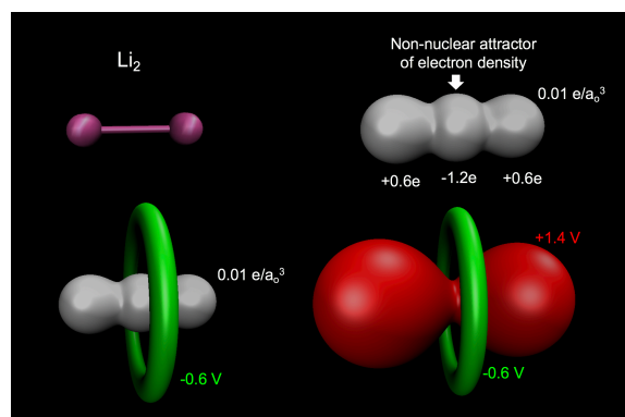
Figure 6: Lithium dimer ( \text{Li}_2 ) displays a NNA in the electron density (white isosurface with 0.01\text{ e}/a_0^3 ) at the midpoint is surrounded by a halo of negative electric potential at -0.6\text{ V} (green), with the entire molecule wrapped in positive electric potential +1.4\text{ V} (red). Bader charges yield that the NNA has a charge of -1.2e with the Li atoms carrying a charge of +0.6e . QM level: B3LYP/6-31+G*
