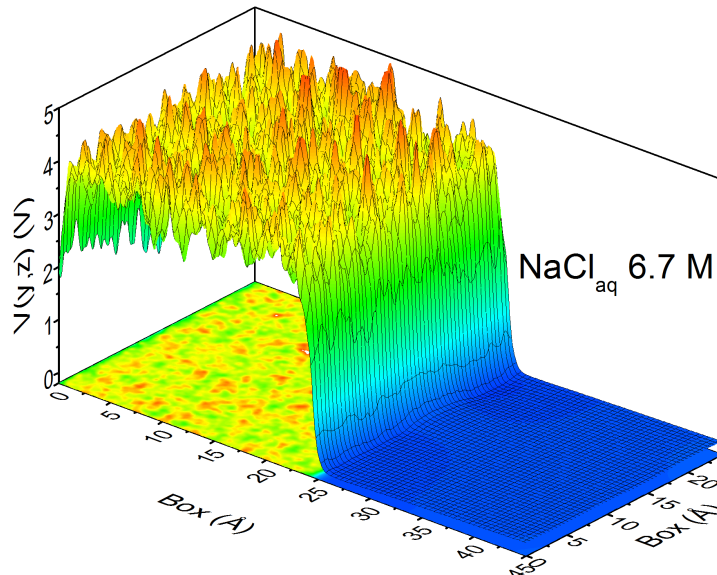
Figure 12: The profile of the electric potential for a slab of 6.7 M aqueous NaCl spanning both the bulk and vacuum regions. QM level: PBE/DZVP.
