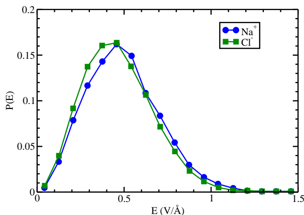
Figure 10: Comparison of electric field distributions at the locations of the \text{Na}^+ and \text{Cl}^- ions from CL simulations of a 6.7 M aqueous NaCl electrolyte.
