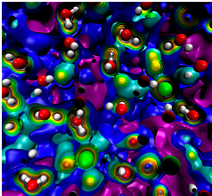
Figure 8: QM electric potential isosurfaces inside 6.7 M aqueous NaCl. Atom colors are: water’s O and H atoms are red and white, respectively, \text{Na}^+ cations are blue, and \text{Cl}^- anions are green. Isosurfaces are: +10.3 V (gray), +6.8 V (orange), +2.7 V (yellow), 0 V (green), -1.4 V (cyan), -3.3 V (blue), -4.6 V (purple). The simulation box length is L = 24.4 \text{ \AA} . QM level: PBE/DZVP
