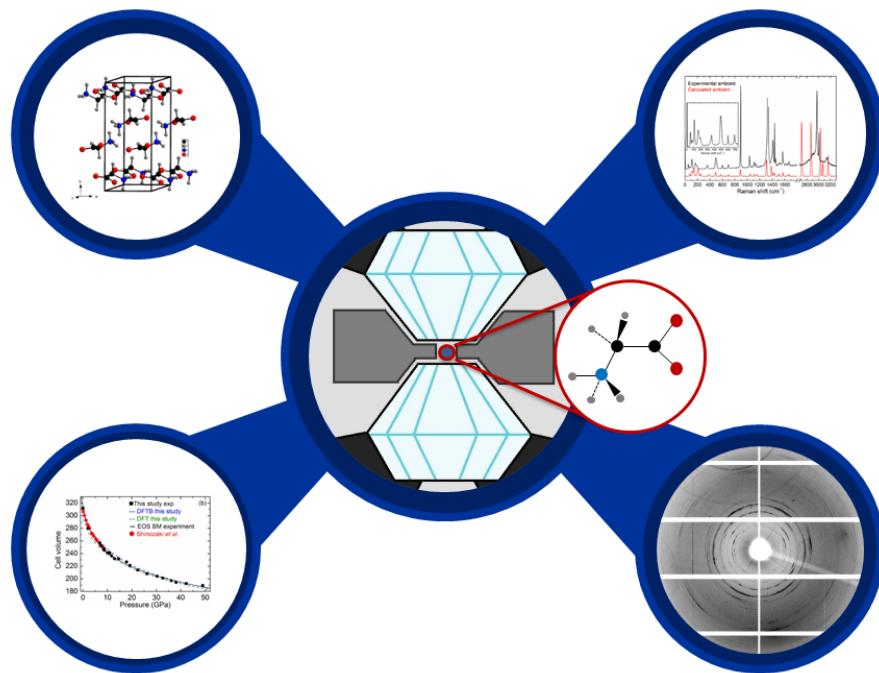
This concomitant experimental and theoretical study provides a definitive EOS for \alpha -glycine up to the record pressure of 50 GPa.
