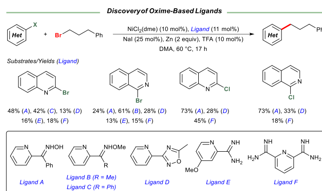
Scheme 5: Discovery of PyOxime Ligands
