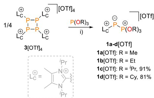
Scheme 1 Nucleophilic fragmentation of 3[\text{OTf}]_4 with organophosphites \text{P(OR)}_3 ( R = \text{Me, Et, } ^i\text{Pr, Cy} ); reagents and conditions: (i) +4.2 \text{P(OR)}_3 , \text{CH}_3\text{CN} or \text{CD}_2\text{Cl}_2 , r.t., 16 h, 91% ( 1\text{c}[\text{OTf}] , R = ^i\text{Pr} ), 16 h, 81% ( 1\text{d}[\text{OTf}] , R = \text{Cy} ).
