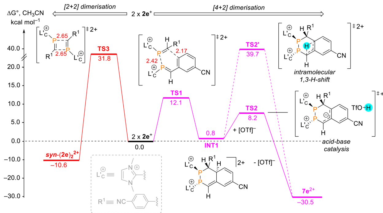
Fig. 6 Calculated free energy profile ( \Delta G^\circ , RI-BP86-D4/def2-TZVP, COSMO = \text{CH}_3\text{CN} ) for the transformation of two equiv. of 2e^+ to 7e^{2+} via a [4 + 2] dimerisation followed by acid-base catalysis (magenta pathway). For comparison, the competing [2 + 2] dimerisation to form \text{syn}-(2e)_2^{2+} (red pathway) is also shown. All energies are reported in \text{kcal mol}^{-1} and are relative to two isolated molecules of 2e^+ . A truncated model for the imidazolium substituent was used for all calculations.
