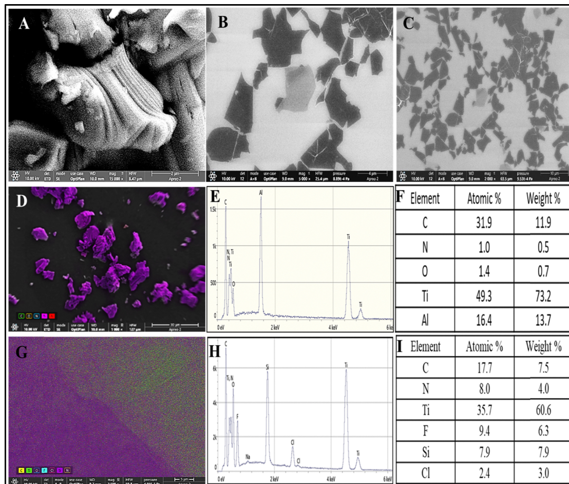
Fig. 2 Microscopic characterization of MXene: HR-SEM for (A) the Max phase ( Ti_3AlC_2X ) and (B) and (C) delaminated MXene sheets ( Ti_3C_2X ); EDS analysis: (D) EDS image, (E) EDS mapping, and (F) elemental composition of the Max phase ( Ti_3AlC_2X ); (G) EDS image, (H) EDS mapping, and (I) elemental composition of delaminated MXene sheets ( Ti_3C_2X ).
