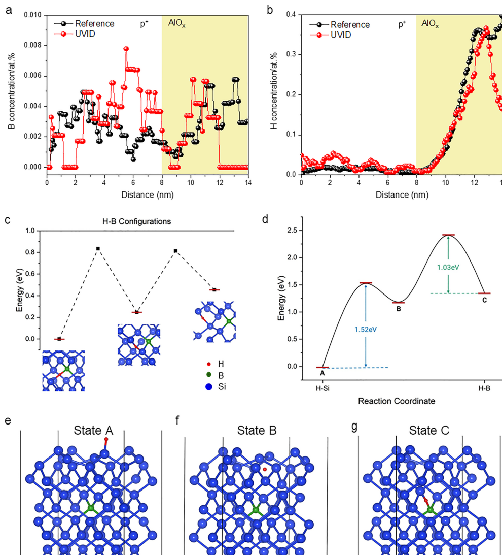
Fig. 4 1-D concentration profile of (a) B and (b) H across the interface of \text{AlO}_x and p^+ region derived from the highlighted area in Fig. S4 in reference and UVID cells (detailed in S4). (c) Three configurations of H-B and their relative system energies. The configuration in which H is located near the centre of the B-Si bond exhibits the lowest energy, indicating the formation of a B-H bond. (d) NEB calculation results, with states A, B and C demonstrated in (e)–(g) respectively. State A corresponds to the configuration where H passivates the Si surface by forming H-Si bonds; State B represents the intermediate state where H penetrates into the subsurface region; and State C denotes the formation of a B-H bond. The sequence A–B–C represents the UVID irradiation process, while the reverse sequence corresponds to the LSIR process.
