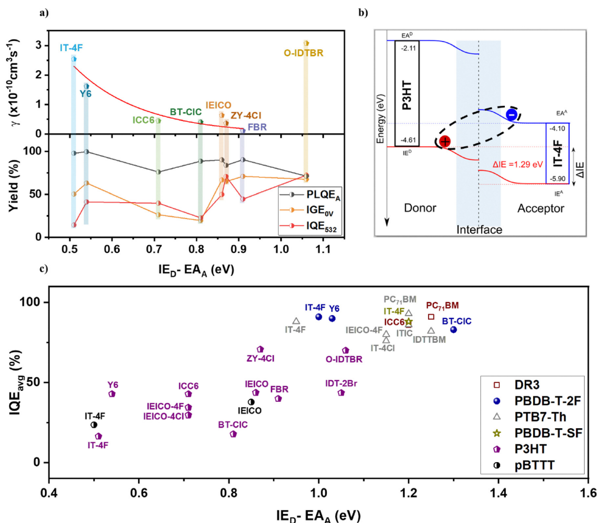
Fig. 8 Impact of diagonal bandgap on non-geminate recombination rates. (a) Bi-molecular recombination rate constant ( \gamma ) as a function of the diagonal bandgap ( |E_D - E_{A\lambda}| ) (top panel) and the evolution of PLQE A , IGE at 0 V, and IQE at 532 nm of the diagonal bandgap (bottom panel). (b) Schematic representation of the diagonal bandgap ( |E_D - E_{A\lambda}| ) at the interfacial landscape between the donor and the acceptor. (c) IQE Avg as a function of diagonal bandgap, based on six different donors paired with various NFAs and a Fullerene acceptor (FA) (PCBM) across 25 systems (IQE Avg of P3HT and pBTTT was obtained from this study, while the other donors were obtained from our previous work 24 ).
