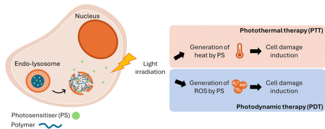
Fig. 7 Schematic illustration of cell damage by PTT and PDT after polymeric nanocarrier endosomal escape and photosensitizer release.
