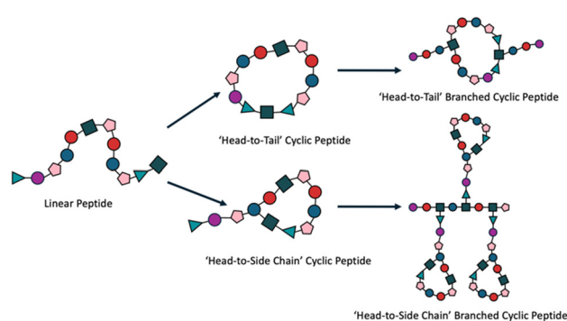
Fig. 5 Generation and incorporation of cyclic peptides into branched peptide systems. The process begins with a linear peptide precursor, which can be cyclised into two distinct types of cyclic peptides: 'head-to-side chain' cyclic peptides, characterised by a cyclical end with a linear tail, and 'head-to-tail' cyclic peptides, featuring a simple closed-ring configuration. These cyclic peptides are subsequently incorporated as branching points into branched peptide systems, enhancing the versatility and stability of the resulting biomaterials.
