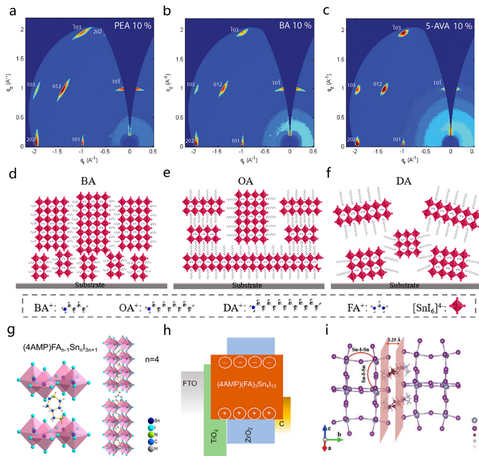
Fig. 10 GIWAXS of (a) PEA 2 FA n-1 Sn n I 3n+1 with 10% NH 4 Cl addition, (b) BA 2 FA n-1 Sn n I 3n+1 with 10% NH 4 Cl addition, and (c) 5-AVA 2 FA n-1 Sn n I 3n+1 with 10% NH 4 Cl addition. 109 Copyright 2019, Wiley-VCH GmbH. Schematic of the crystal orientation, size and phase distribution of two-dimensional perovskite thin films: (d) BA, (e) OA, and (f) DA. 81 Copyright 2020, the American Chemical Society. (g) Schematic of the crystal structure of DJ-phase Sn-based halide perovskites (4AMP)(FA) n-1 Sn n I 3n+1 (n = 4). 110 Copyright 2019, the American Chemical Society. (h) Energy-level diagram of HTML-free PSC based on DJ Sn(II). 110 Copyright 2019, the American Chemical Society. (i) Illustration of the distance between the diffraction planes of (BEA)FA n-1 Sn n I 3n+1 . 30 Copyright 2020, Wiley-VCH GmbH.
