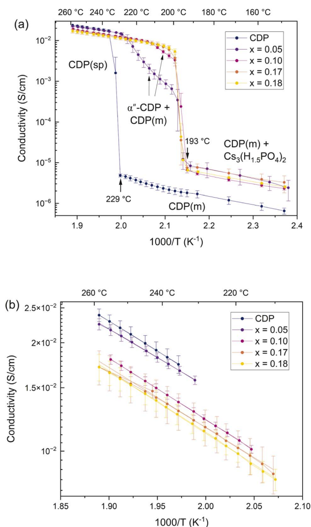
Fig. 8 Conductivities of representative materials in the (1 - x) \text{CsH}_2\text{PO}_4 - x\text{Cs}_2\text{HPO}_4 system collected under p\text{H}_2\text{O} = 0.4 atm: (a) Arrhenius presentation showing behavior over the temperature range 150–260 °C; and (b) behavior in the superprotonic phase space.
